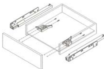
3 sided drawer
