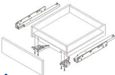
4 sided drawer
